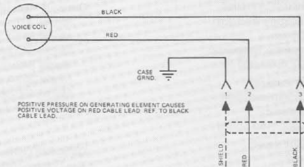
FIGURE 2 - Wiring Diagram
