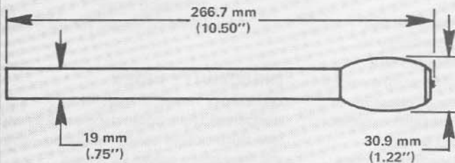
FIGURE 3 - Dimensions
