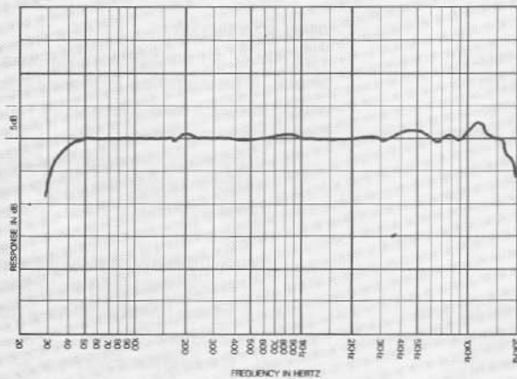
FIGURE 1 - Axial Response
