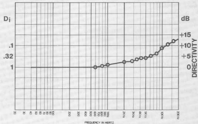
FIGURE 4 - Directivity Index
